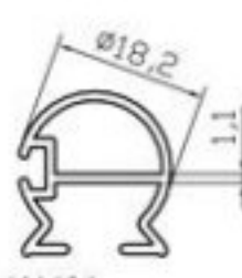
K4401 FİTİLLİ DİKME (0.215 Kg/m)
