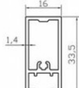
K4406 ASKILIK PROFİLİ (0.430 Kg/m)
