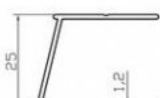
K4413 GÖNYELİ DUVAR DİKME (0.260 Kg/m)
