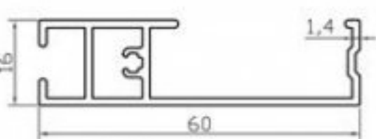
K4408 ASKILIK PROFİLİ (0.540 Kg/m)
