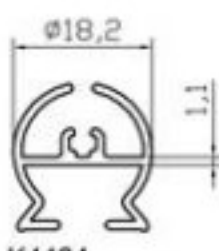
K4424 ARA FİTİLLİ DİKME (0.245 Kg/m)
