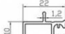
K4419 FİTİLSİZ DİKME (0.300 Kg/m)
