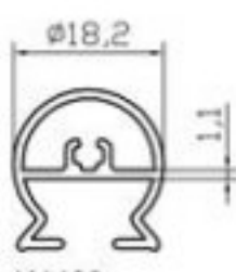
K4400 FİTİLSİZ DİKME (0.215 Kg/m)
